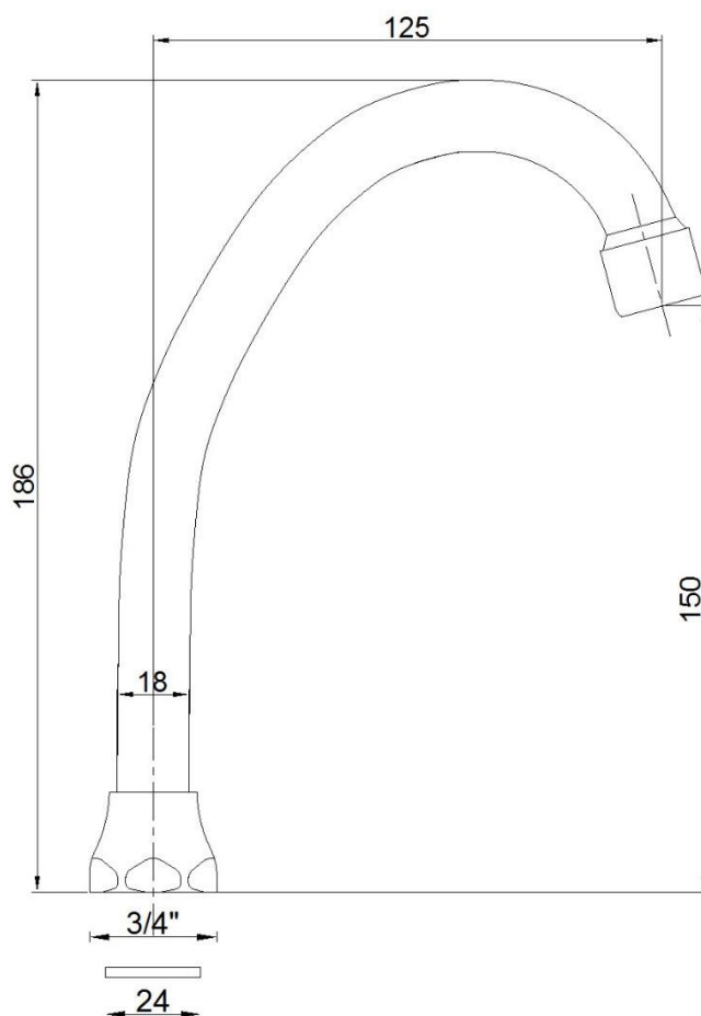
Attacco universale 3/4"
